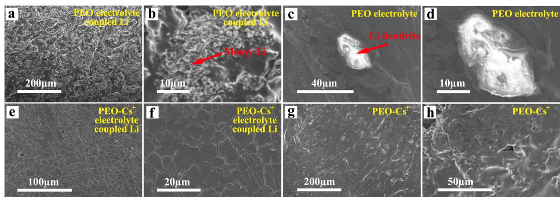
Figure 3. SEM images of (a)~(b) PEO electrolyte-based Li and (c)~(d) PEO electrolyte after 100 h; SEM images of (e)~(f) PEO-Cs + electrolyte based Li and (g)~(h) PEO-Cs + electrolyte after 100 h.
