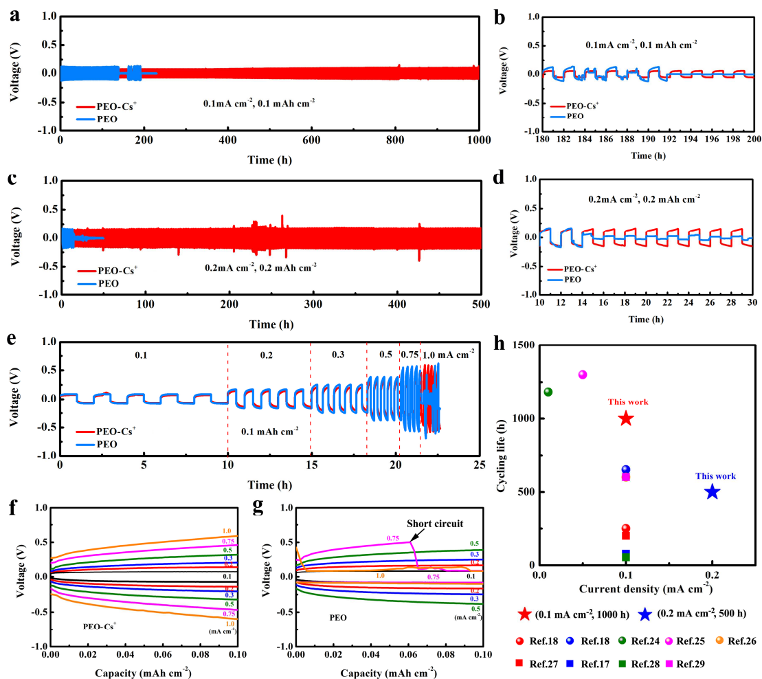
Figure 2. Comparison of the cycling stability of the Li-Li symmetrical cells assembled with PEO- \text{Cs}^+ and PEO electrolyte at (a-b) 0.1 \text{ mA cm}^{-2} (capacity: 0.1 \text{ mAh cm}^{-2} ) and (c-d) 0.2 \text{ mA cm}^{-2} (capacity: 0.2 \text{ mAh cm}^{-2} ). (e) Rate performance of the Li-Li symmetrical cells assembled with PEO- \text{Cs}^+ and PEO electrolytes at various current densities of 0.1 to 1 \text{ mA cm}^{-2} with a limited capacity of 0.1 \text{ mAh cm}^{-2} . Relatively plating/stripping profiles of (f) PEO- \text{Cs}^+ electrolyte and (g) PEO electrolyte. (h) Comparison of the recently reported plating/stripping performances of SPEs-based Li-Li symmetric cells with respect to current density and cycling life.
