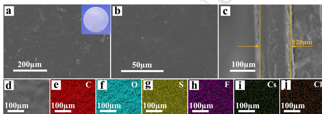
Figure 1. (a)~(b) Surface and (c) cross-sectional morphology of PEO-Cs + electrolyte at different magnifications. (d) SEM image and corresponding elemental mappings of (e) C, (f) O, (g) S, (h) F, (i) Cs and (j) Cl. Inset of (a) is the optical image of PEO-Cs + electrolyte.
